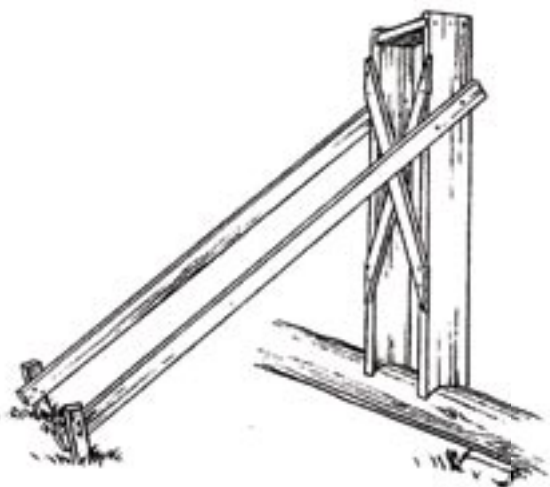
Fig. 29. Door frame set and properly braced.
